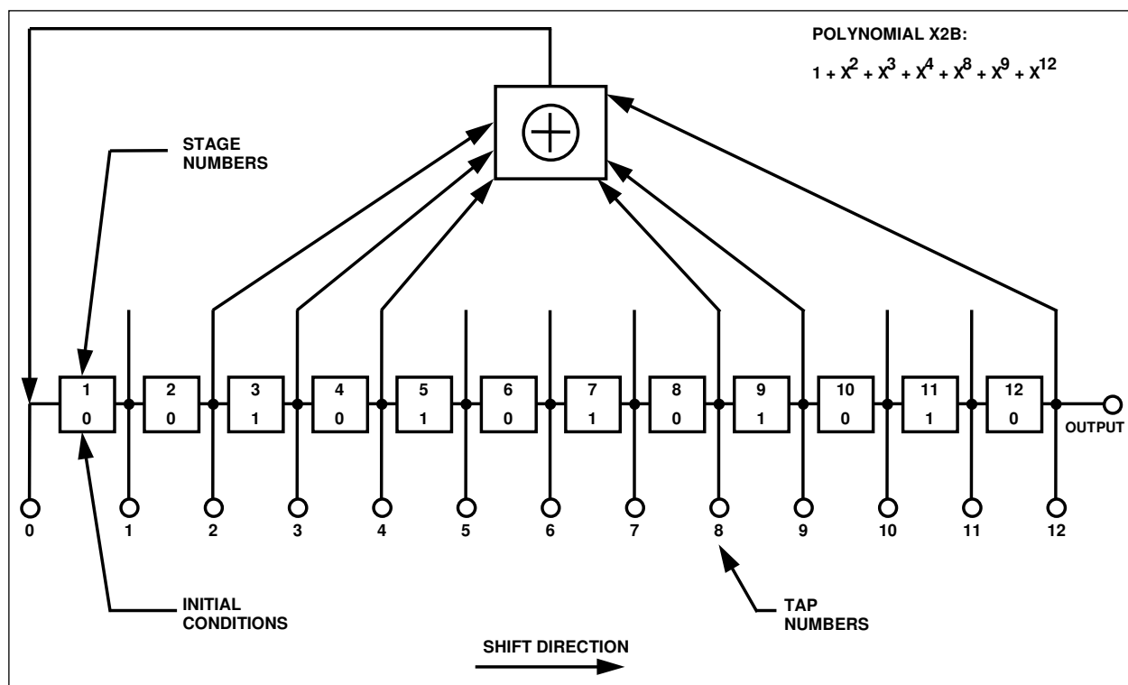
Figure 3-5. X2B Shift Register Generator Configuration
