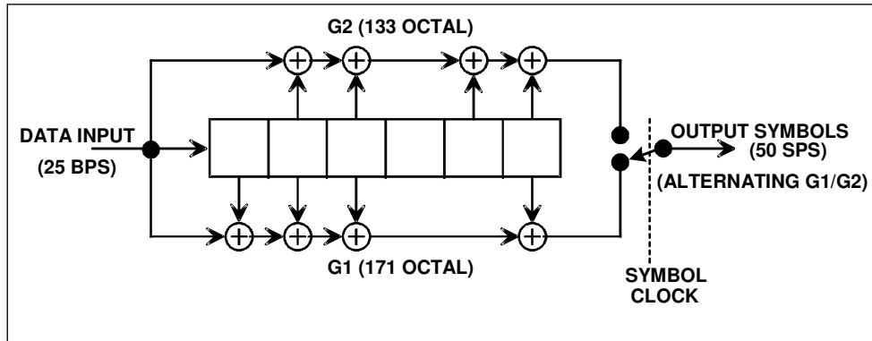
Figure 3-14. Convolutional Encoder
